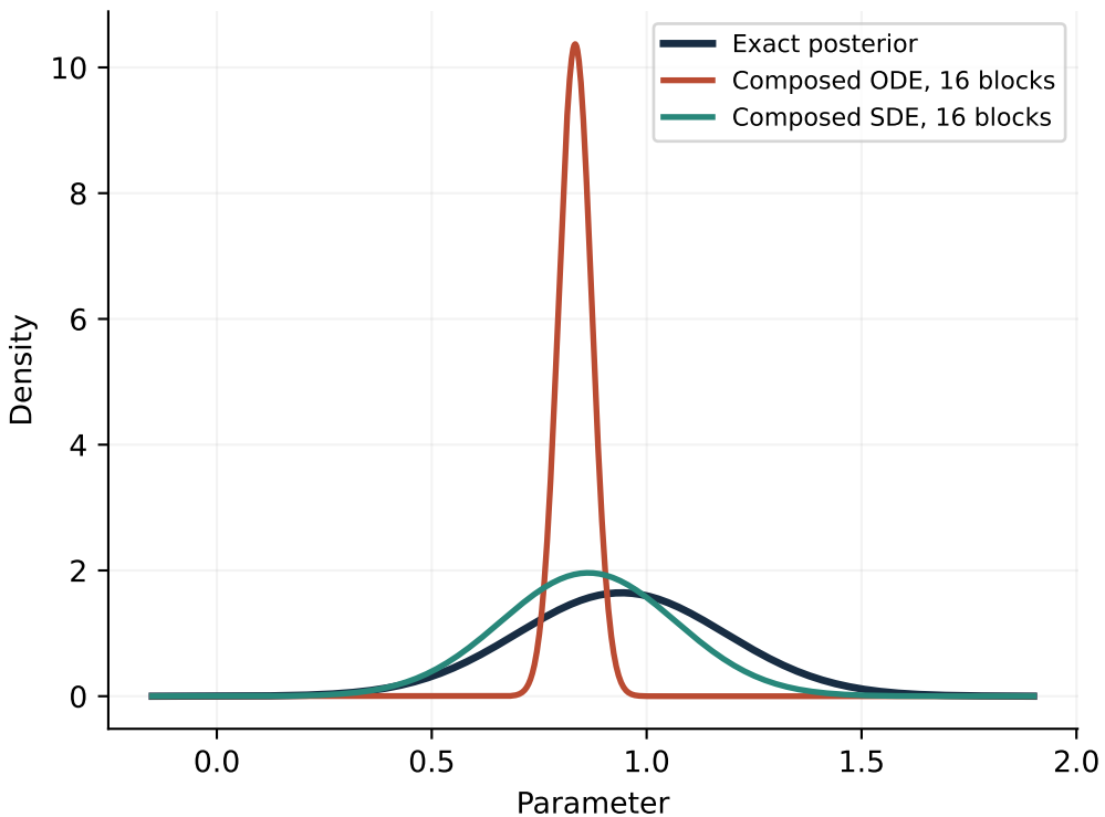
Perfect local scores; 16 observations
