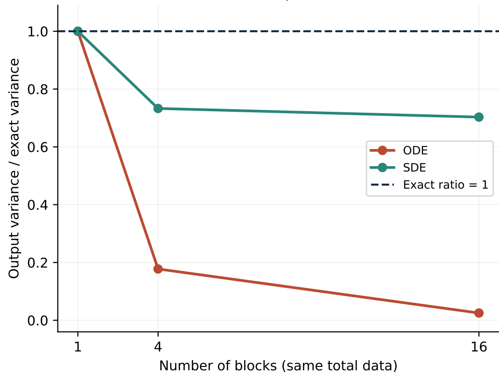
Partition dependence
