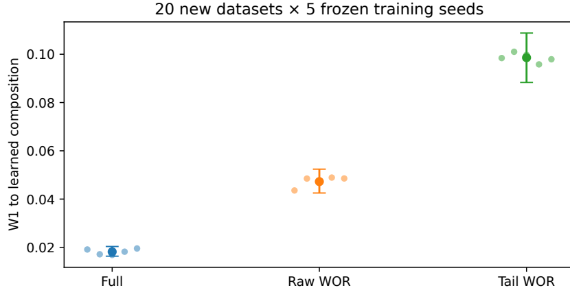
Figure 8: New learned-density replication. Large points show overall means with crossed-bootstrap 95% intervals; five smaller points show the means for individual training seeds, each averaged over the same 20 datasets. Raw WOR has an infinite population normalizer throughout, whereas Full and Tail WOR are finite throughout.
