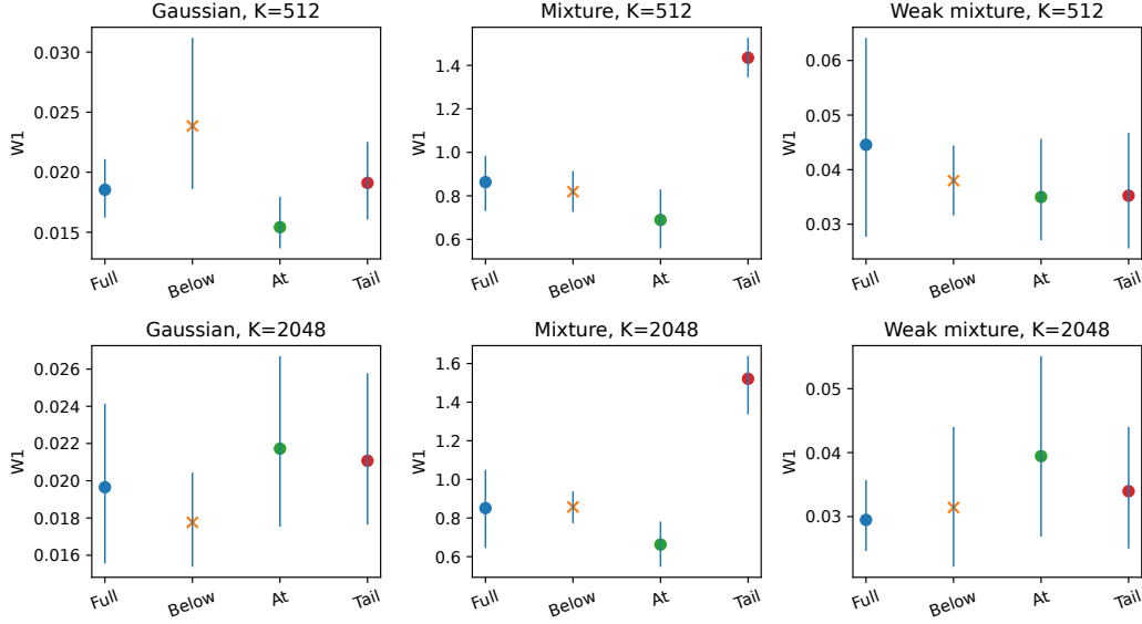
Figure 9: All six boundary comparisons, each with ten sampling seeds. Points show means and vertical bars show bootstrap 95% intervals. Circles denote finite normalizers and crosses infinite ones. Panel-specific vertical scales retain the differences in error magnitude between families.
