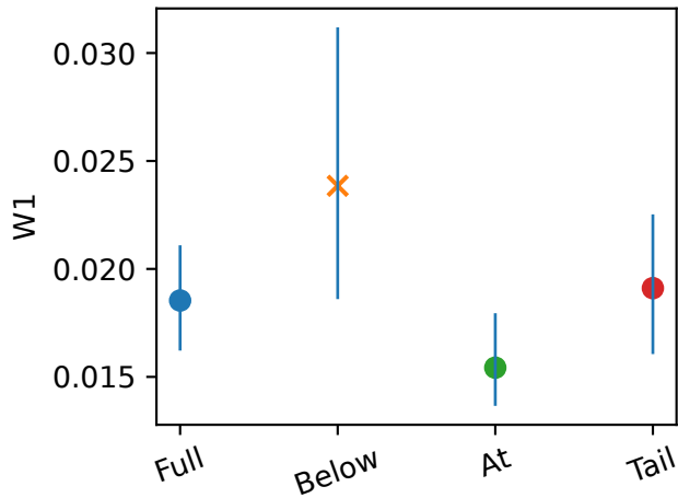
gaussian, K=512
