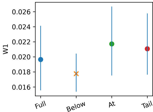
gaussian, K=2048
