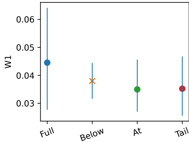
weak_mixture, K=512
