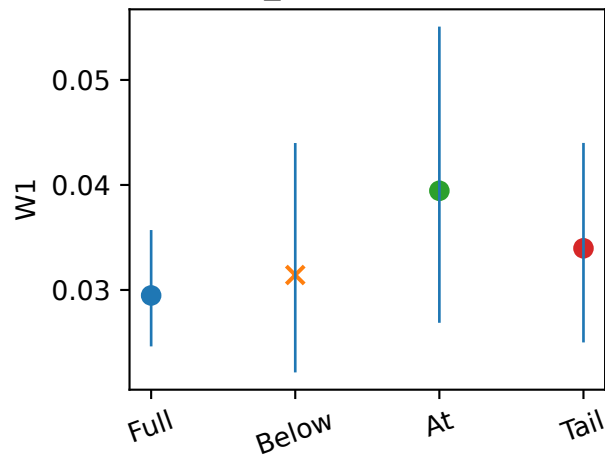
weak_mixture, K=2048
