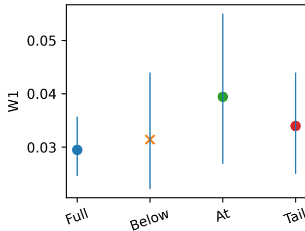
Weak mixture, K=2048
