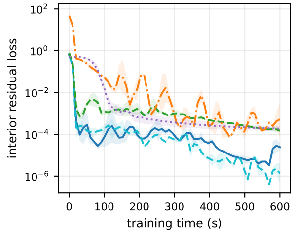
(c) loss vs time ( m = 2 )
