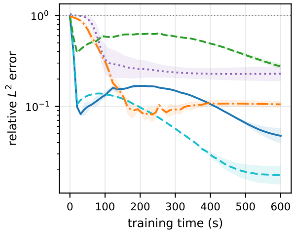
(b) accuracy vs time ( m = 2 )
