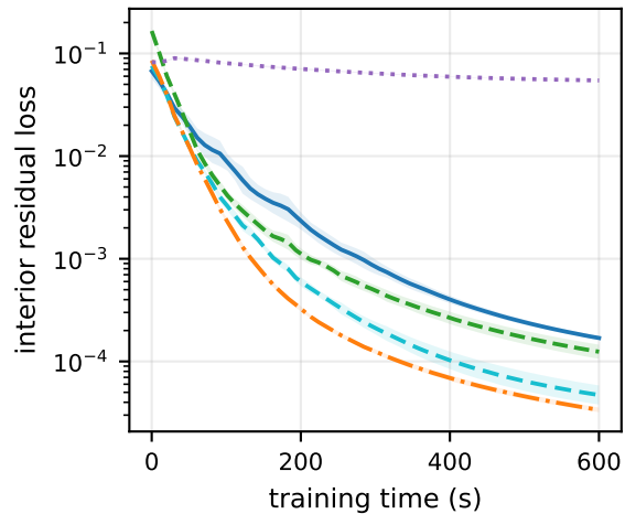
(c) loss vs time ( a = 4 )
