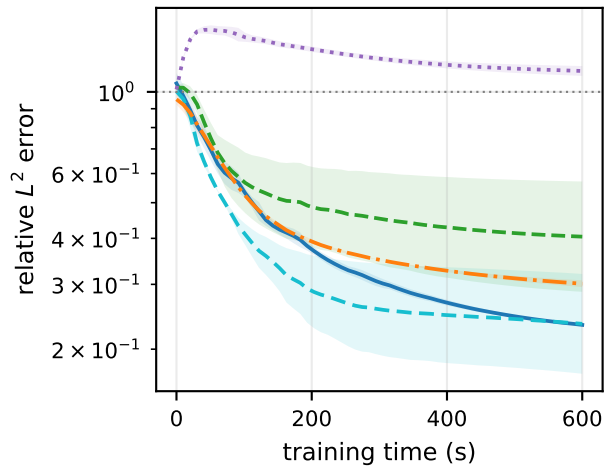
(b) accuracy vs time ( a = 4 )
