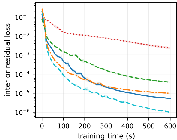
(c) loss vs time ( k = 2 )
