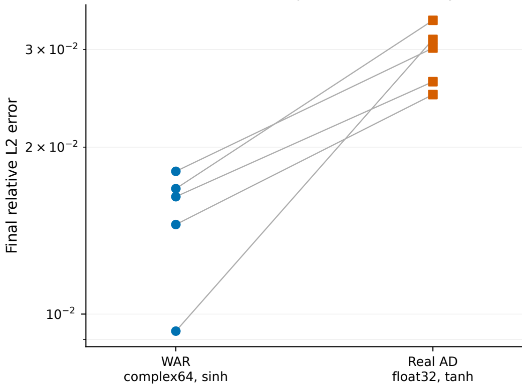
2D third-order ZK: paired final accuracy
