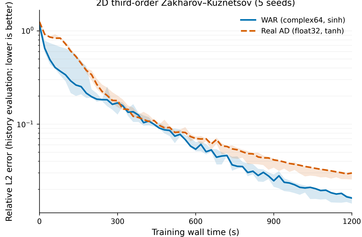
2D third-order Zakharov-Kuznetsov (5 seeds)
