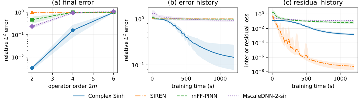
Figure 2: Three-dimensional polyharmonic benchmark, with the same convention as Fig. 1. History panels use the fourth-order configuration.
