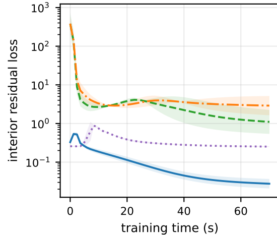
(c) loss vs time (6th order, a = 2 )
