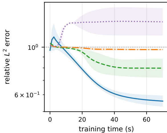
(b) accuracy vs time (6th order, a = 2 )
