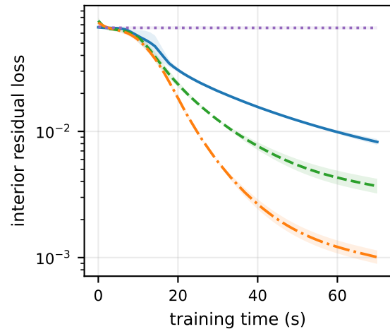
(c) loss vs time ( a = 6 )
