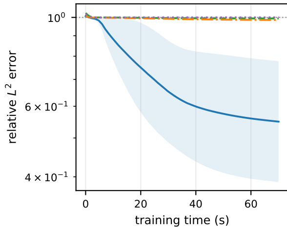
(b) accuracy vs time (modes (3, 4))
