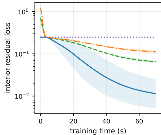
(c) loss vs time (modes (3, 4))
