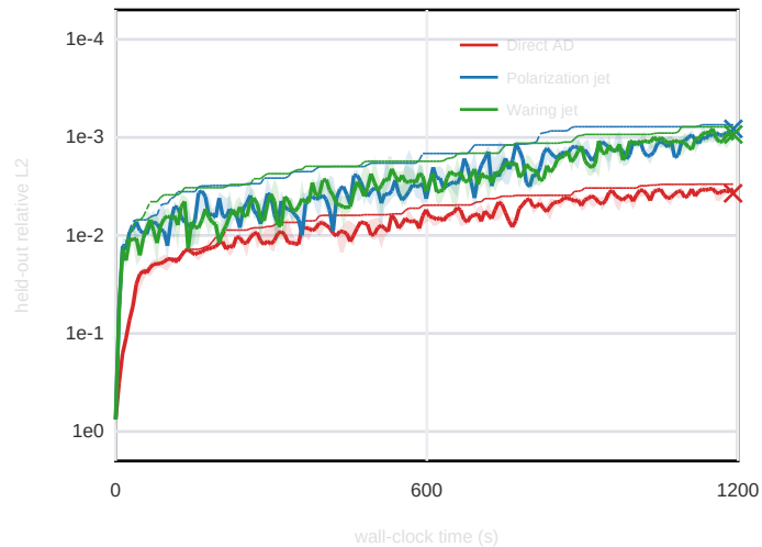
(a) 4D mixed derivative PINN
