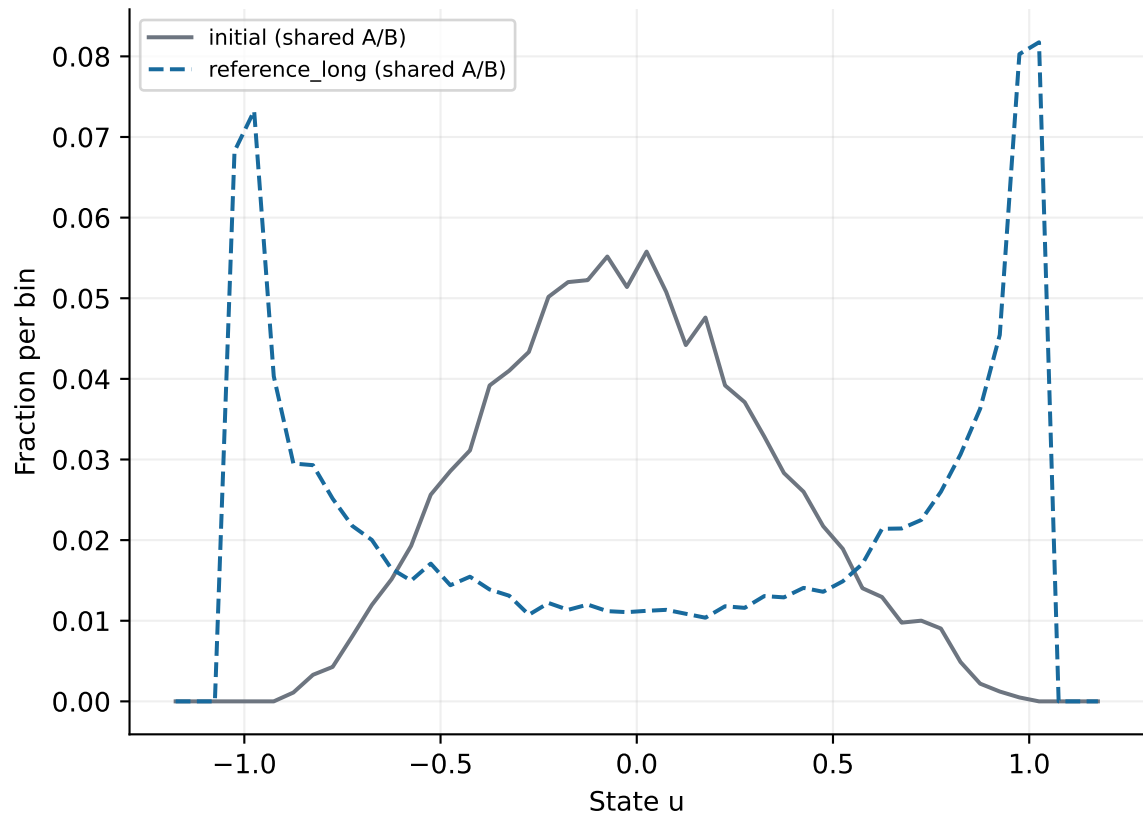
Previous experiment: state distributions, seed 31415
