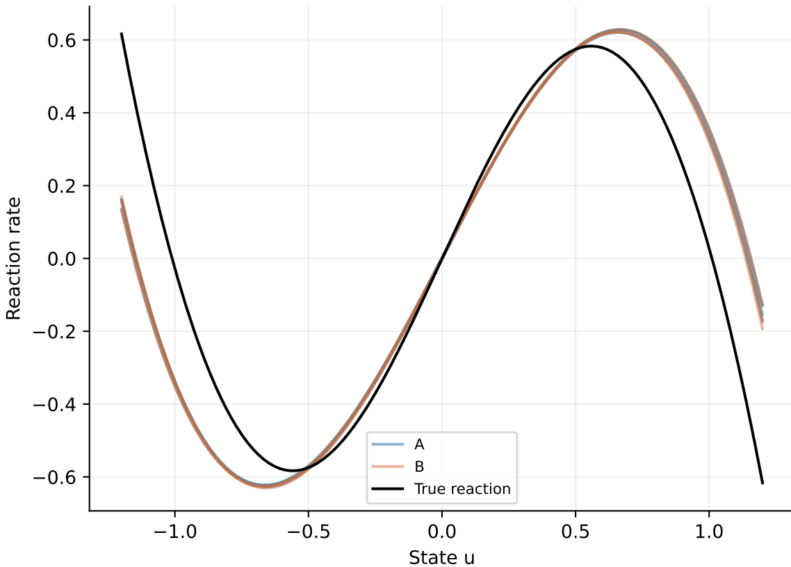
Previous 120-update models: reaction curves
