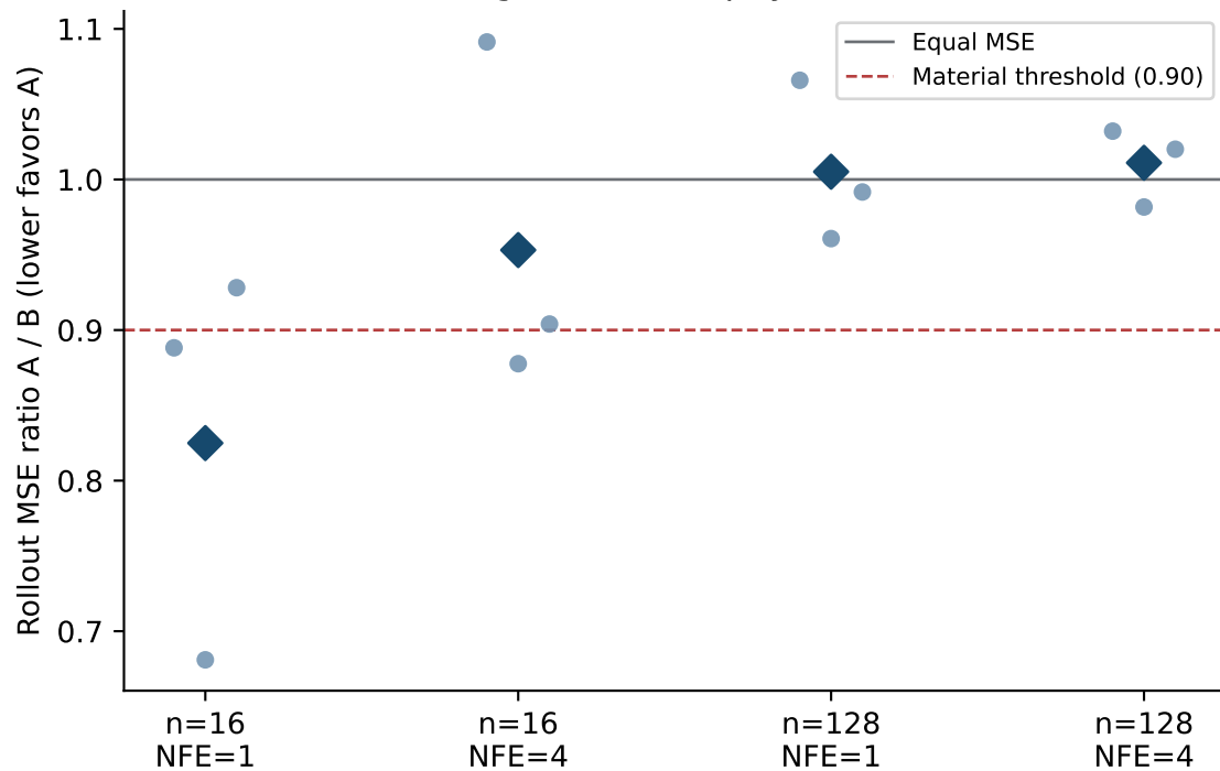
Unseen lags: matched physics and work
