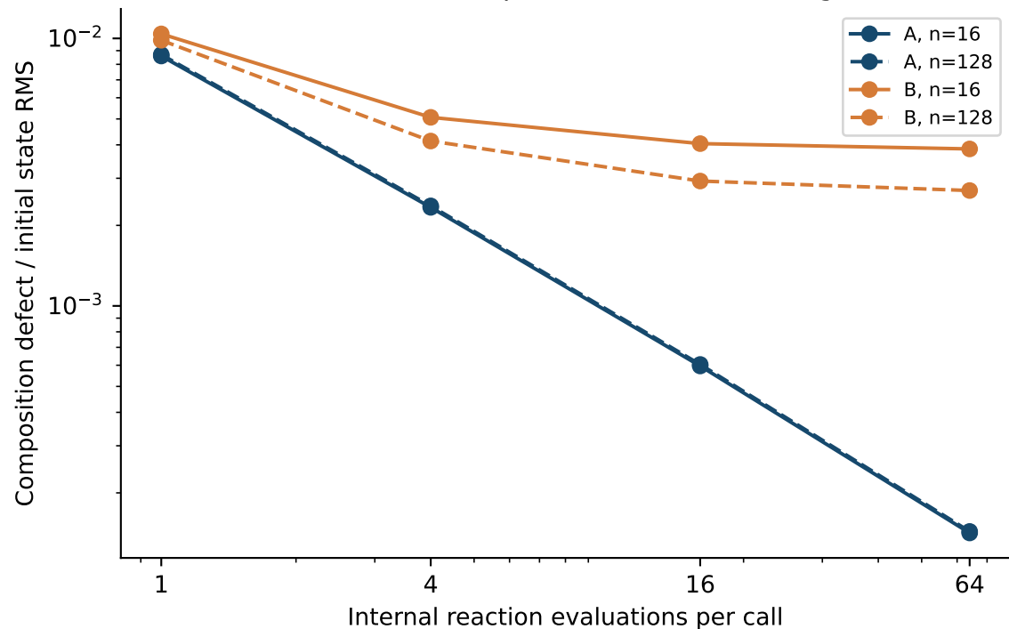
Frozen NFE=4 checkpoints: refinement diagnostic
