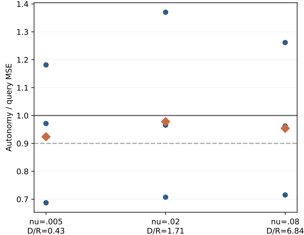
High-frequency OOD, training noise=0.01
