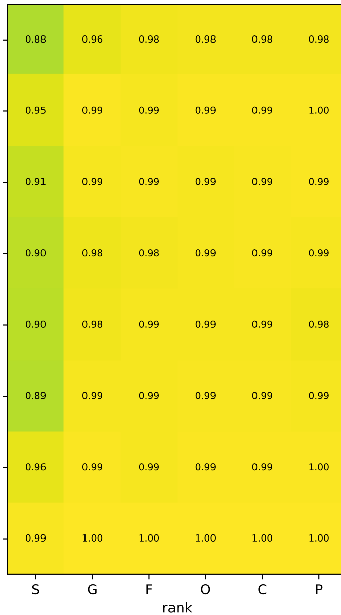
consensus concordance
