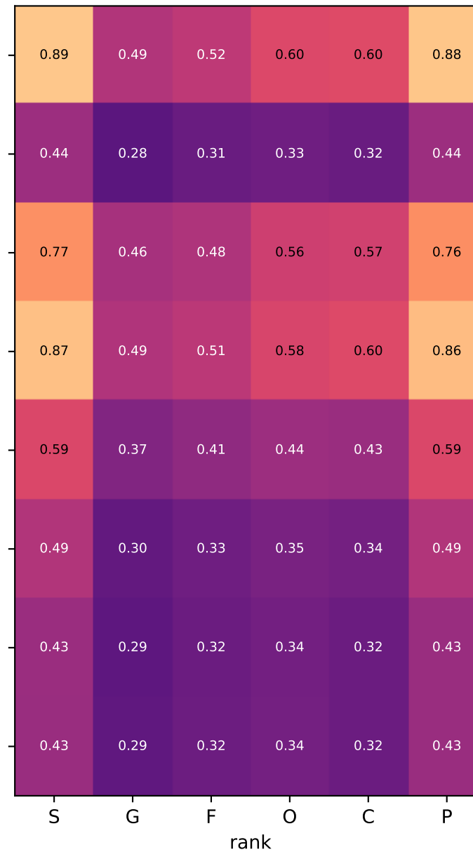
anchor coverage
