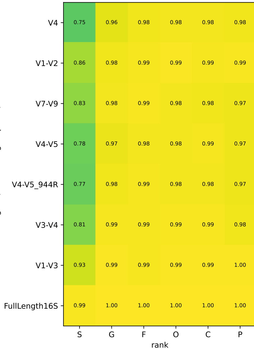
anchor concordance
