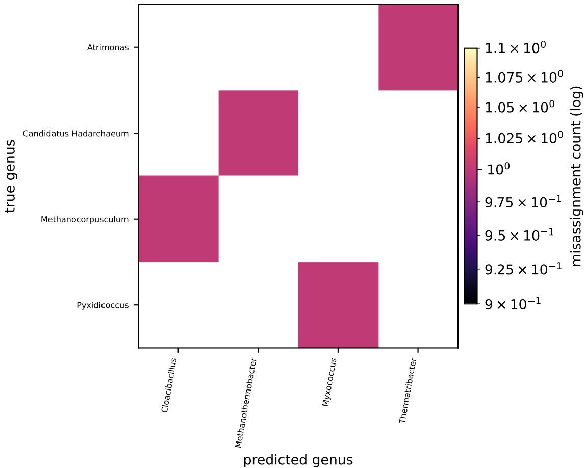
F7 · Genus-failure confusion — V4-V5_944R (anchor, include-self)
