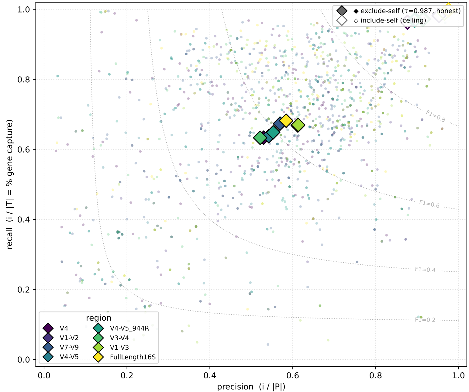
F8 · Recall-precision per amplicon (primary=exclude_0.987); ◆ region centroid
