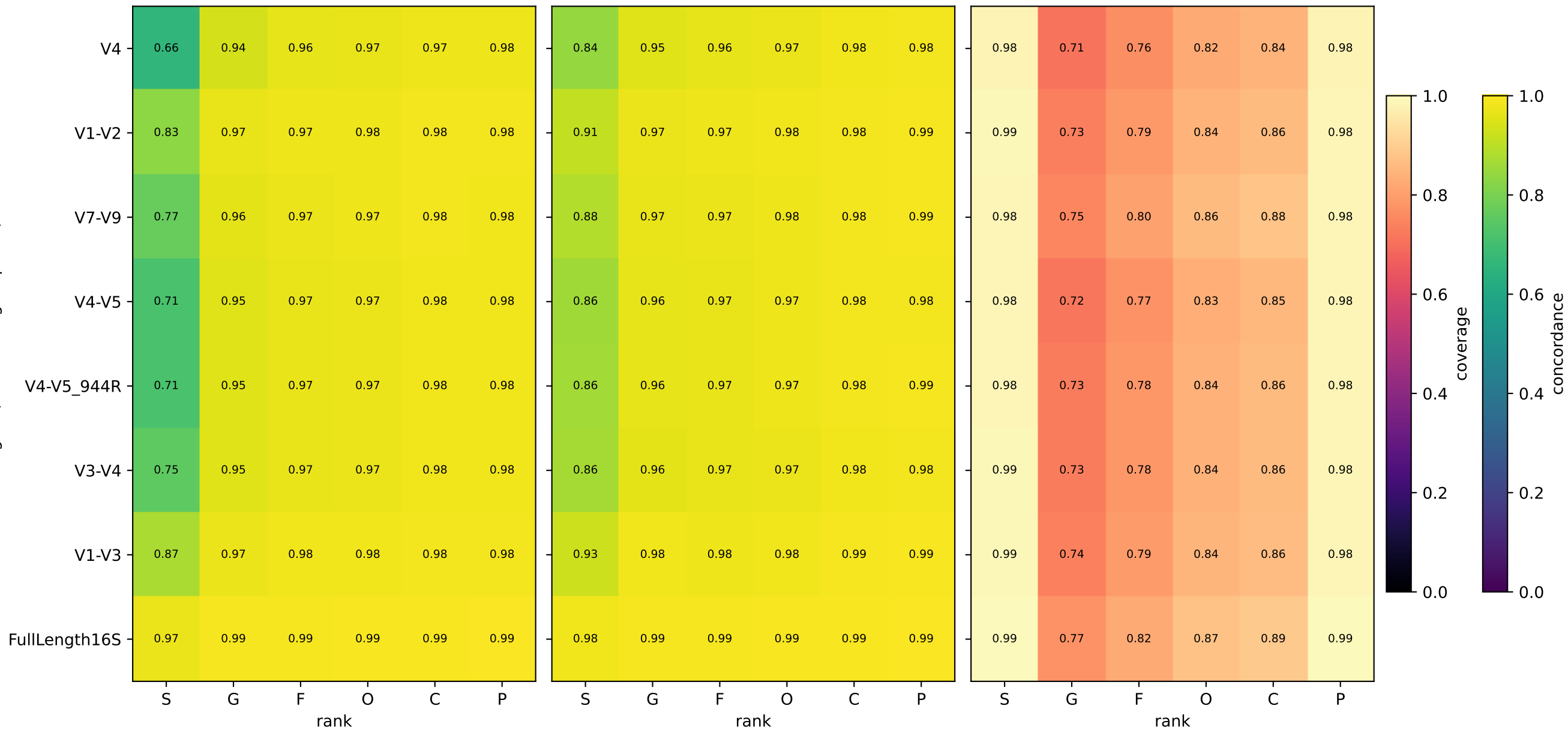
anchor concordance
