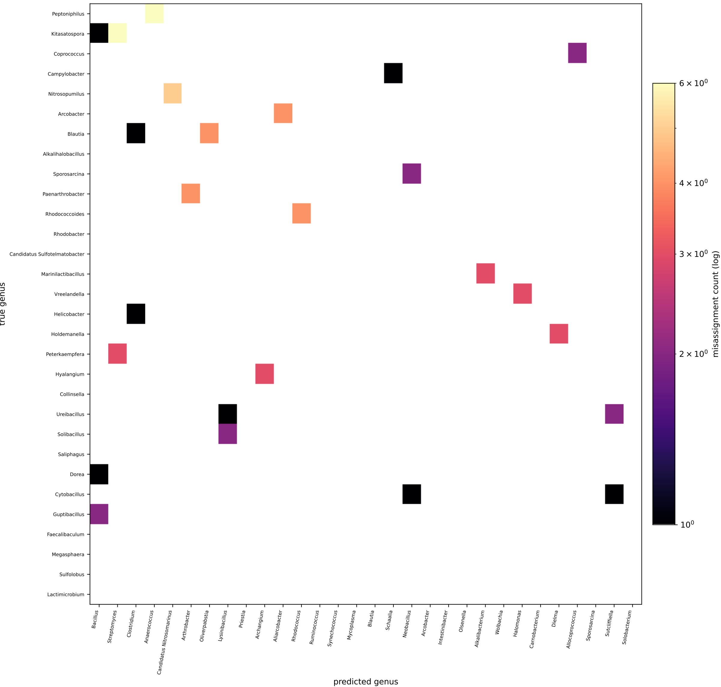
F7 · Genus-failure confusion — V4 (anchor, include-self)
