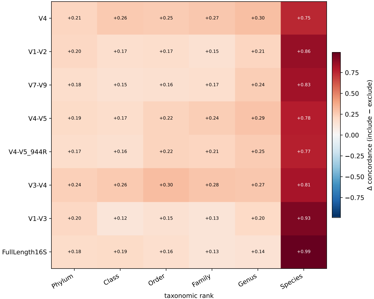
F11 · Include—exclude self concordance \Delta (leakage / generalization gap; anchor)
