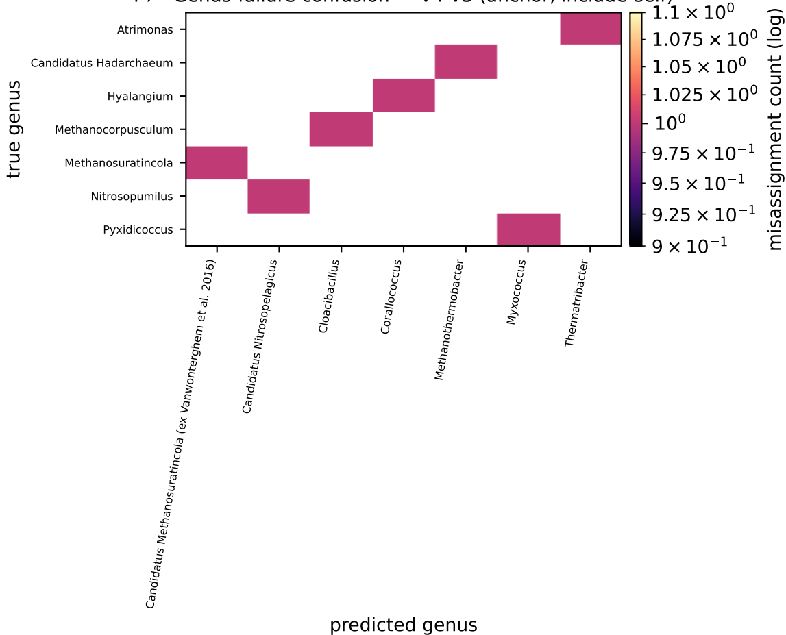
F7 · Genus-failure confusion — V4-V5 (anchor, include-self)
