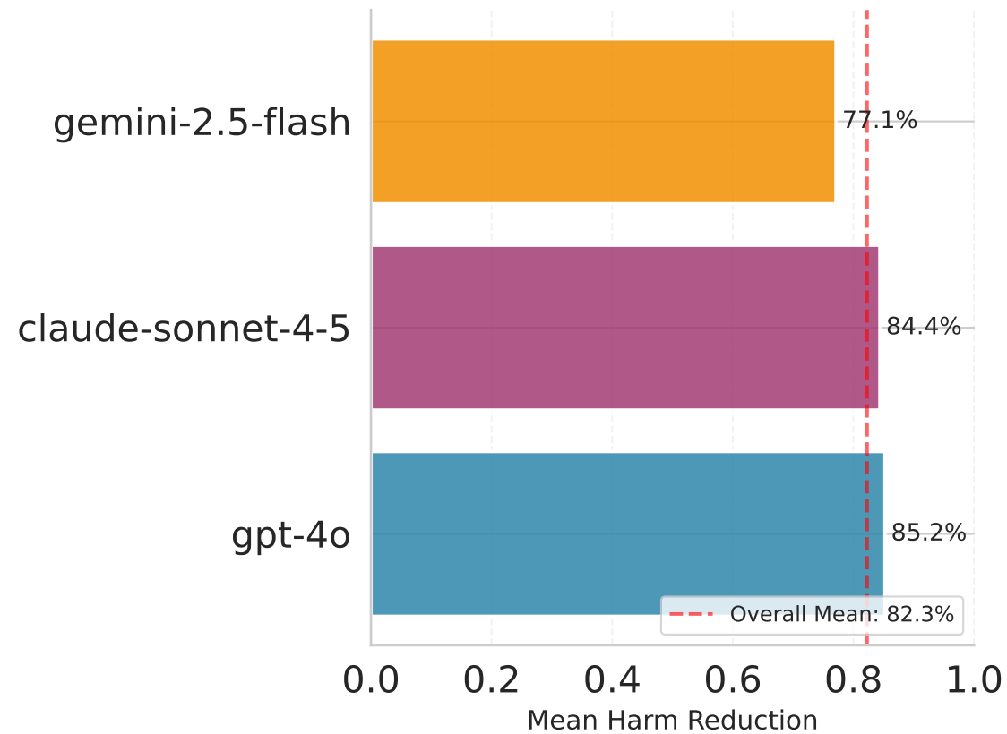
Average Effectiveness by Monitor
