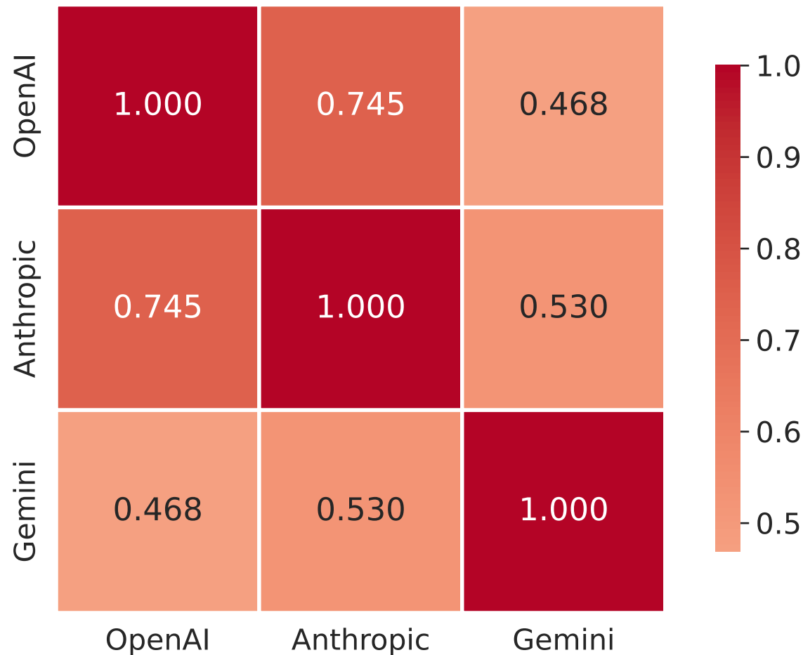
Pearson Correlation Matrix Attack Evaluation Scores
