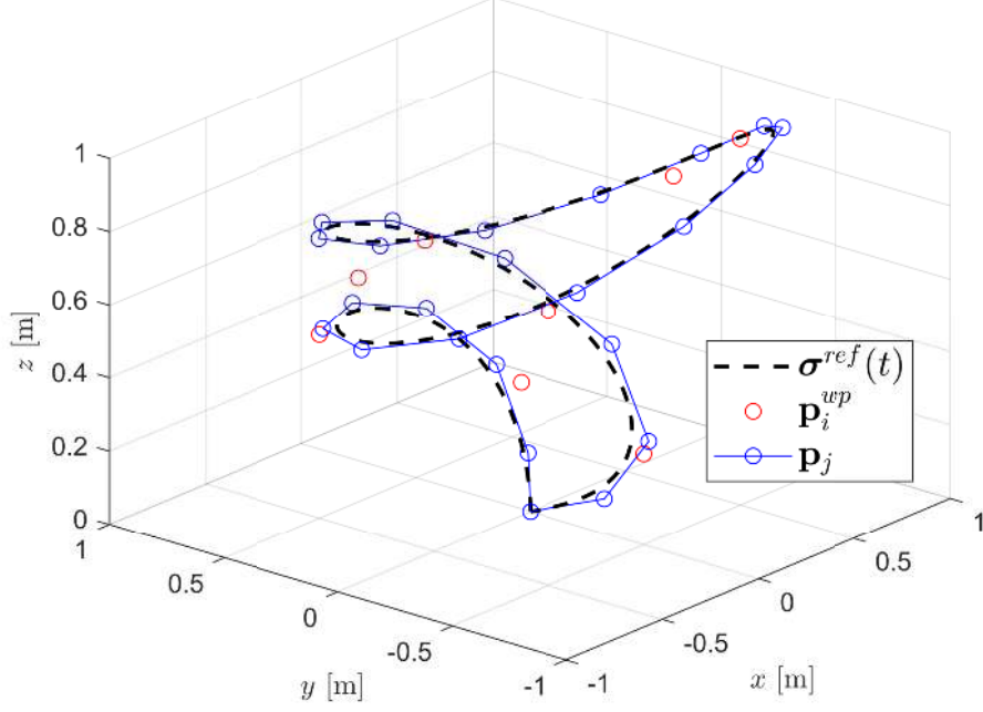
Figure 3.2: The position trajectory generated with the parameters in Table 3.2. We show the position trajectory (dashed black) along with the waypoints (red circles) and the control points (connected, blue circles).
