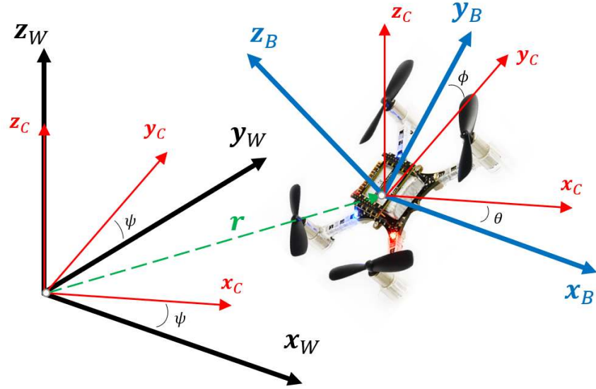
Figure 3.1: Inertial (or world) coordinate frame W (black) and body coordinate frame B (blue). The intermediate coordinate frame C (red) is also shown. Crazyflie2.1 figure from [30].
