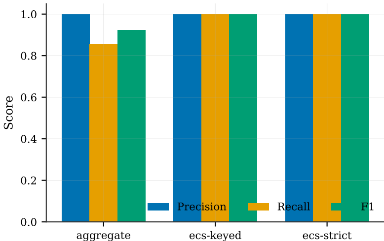
Leave-one-resolver-policy-out (training-benign Q_{0.995} threshold)
