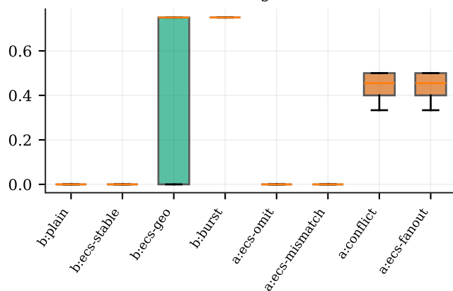
answer disagreement
