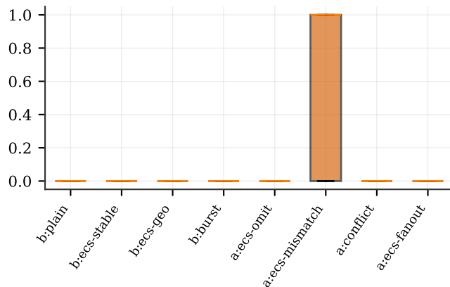
answer disagreement
