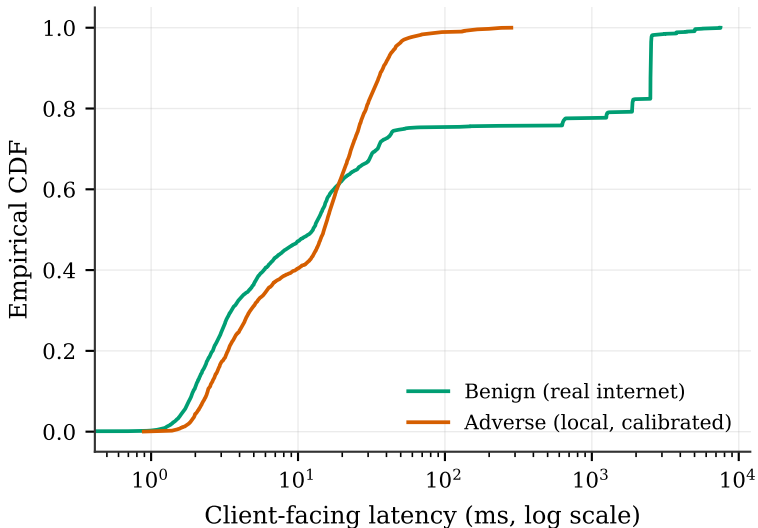
Client latency: benign vs. adverse episodes
