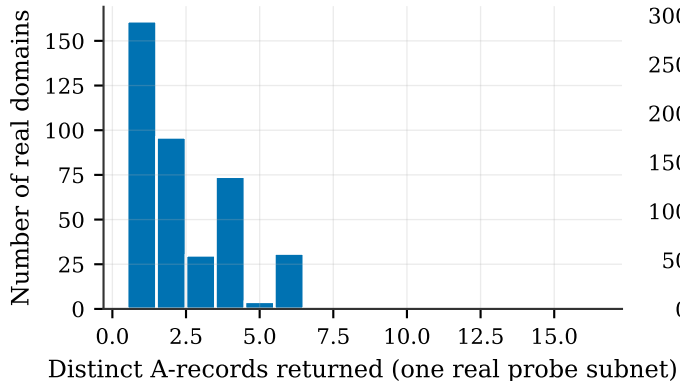
Real answer-set cardinality
