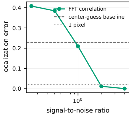
(c) pattern matching = FFT correlation
