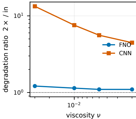
(b) resolution fragility
