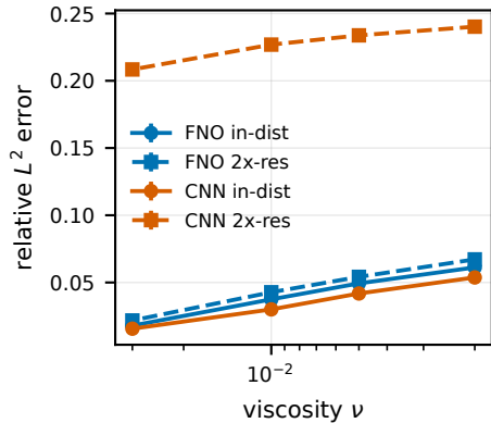
(a) accuracy: in-dist vs 2x resolution
