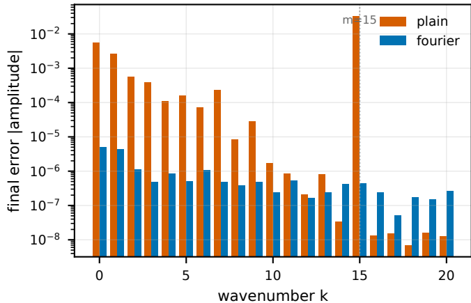
(b) plain misses the high mode; Fourier does not
