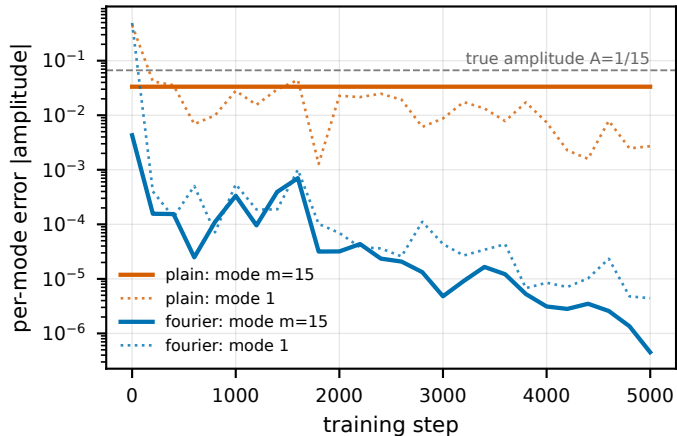
(a) spectral bias: high mode converges slowly
