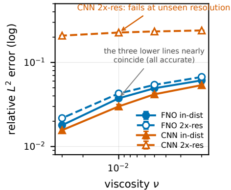
(a) accuracy: in-dist vs 2x resolution
