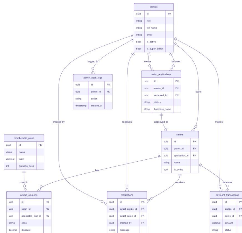
Figure 5.6.3-1. Entity Relationship Diagram (Admin Module)
