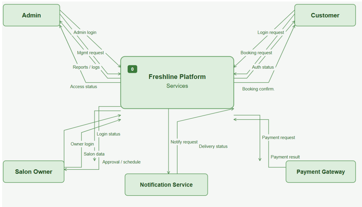
Figure 5.6-1. Data Flow Diagram Level 0
