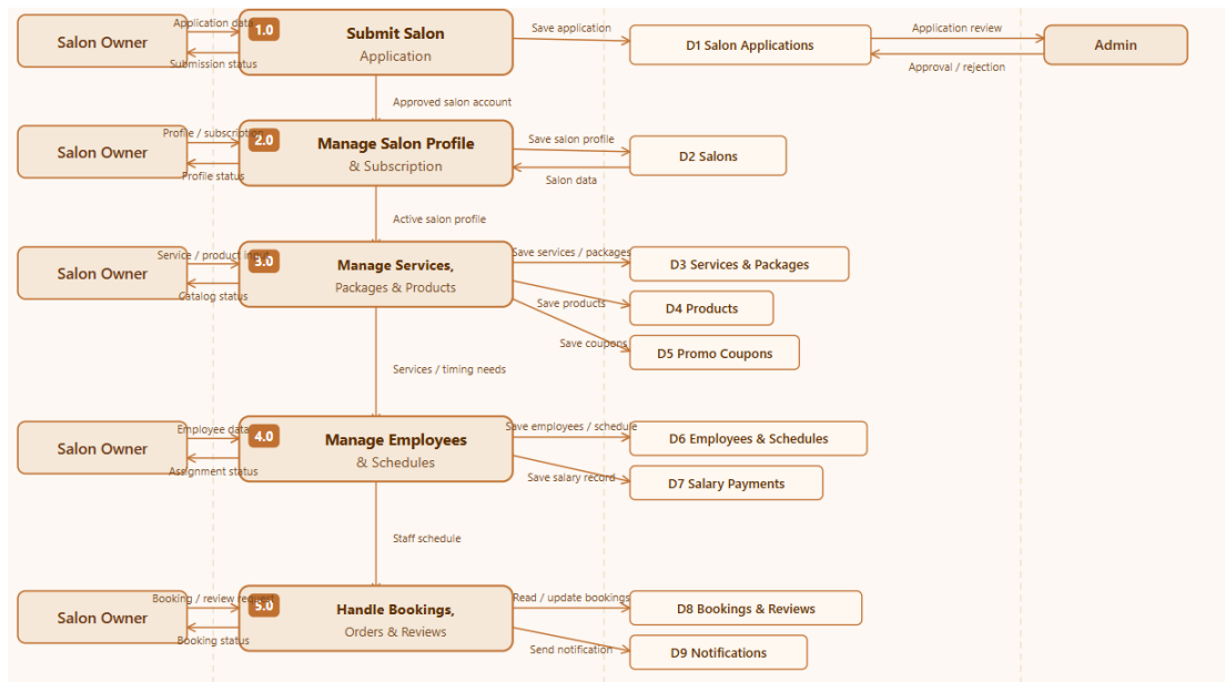
Figure 5.6-3. Data Flow Diagram Level 1 (Salon Owner Module)
