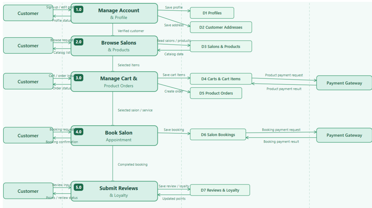
Figure 5.6-2. Data Flow Diagram Level 1 (Customer Module)
