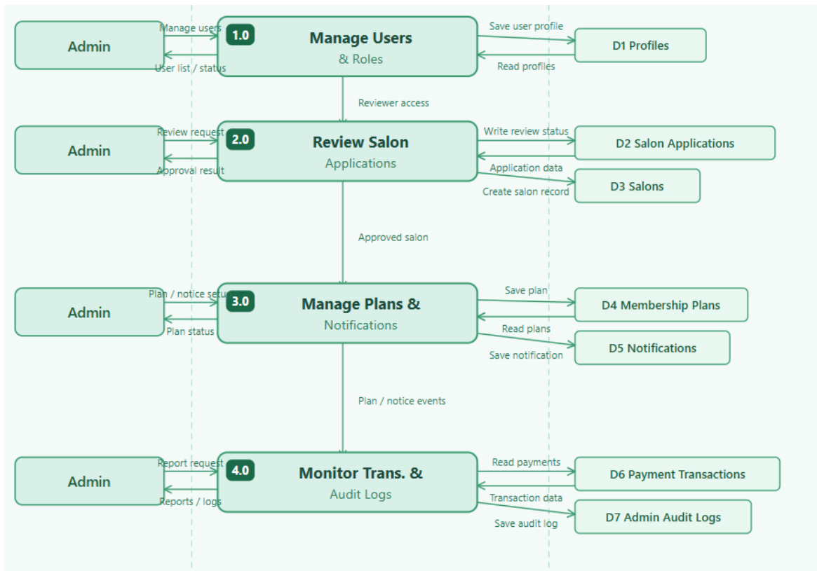
Figure 5.6-4. Data Flow Diagram Level 1 (Admin Module)
