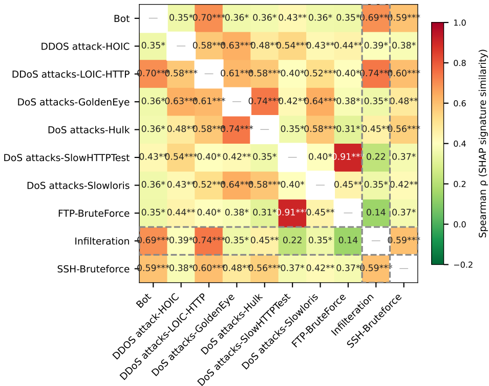
(CIC) Pairwise SHAP signature similarity mean \rho = 0.475 , 4% of pairs \rho < 0.30
