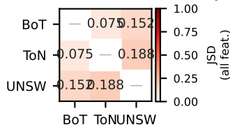
(c) Reconnaissance JSD [All]
