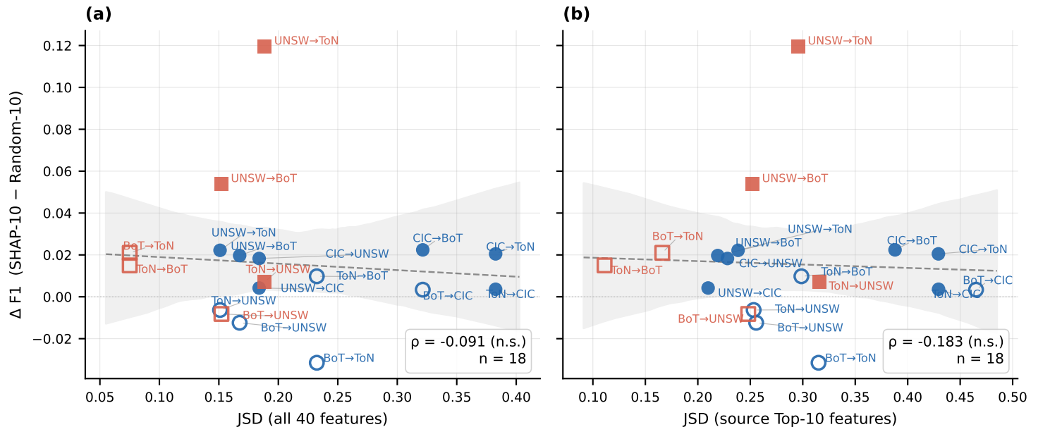
Fig. 10. Jensen-Shannon divergence vs. SHAP-10 transfer performance gain ( \Delta F1 )
