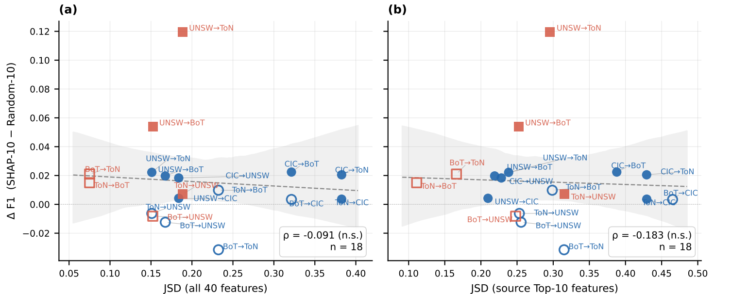
Figure 10. Jensen-Shannon divergence vs. SHAP-10 transfer performance gain ( \Delta F1 )
