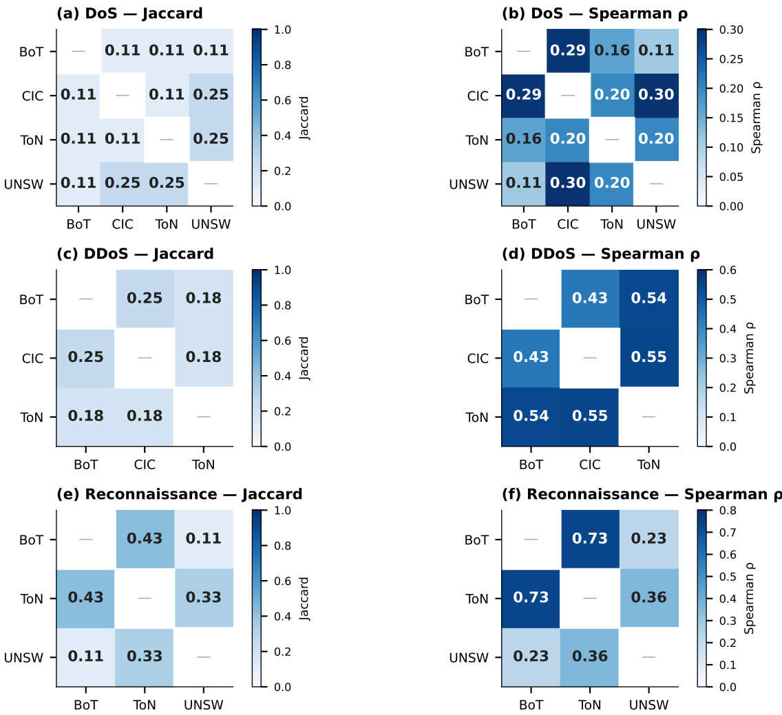
Figure 4. Cross-dataset transferability of SHAP attack signatures (diagonal suppressed; Spearman color scale adjusted to data range)
