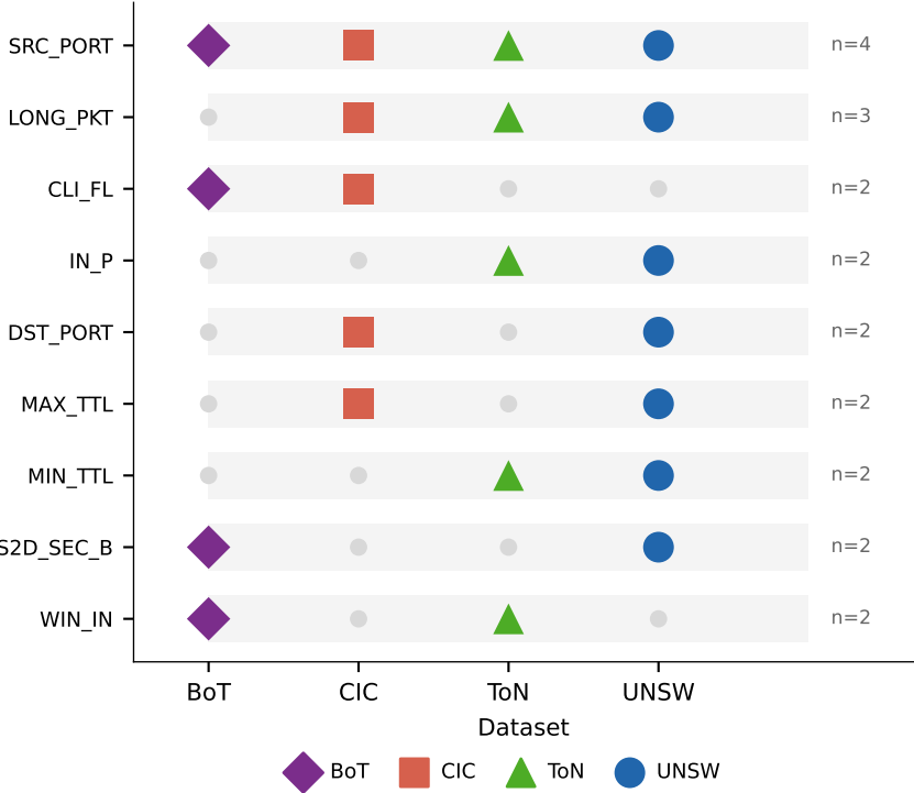
(a) Shared DoS features (appearing in \geq 2 datasets)
