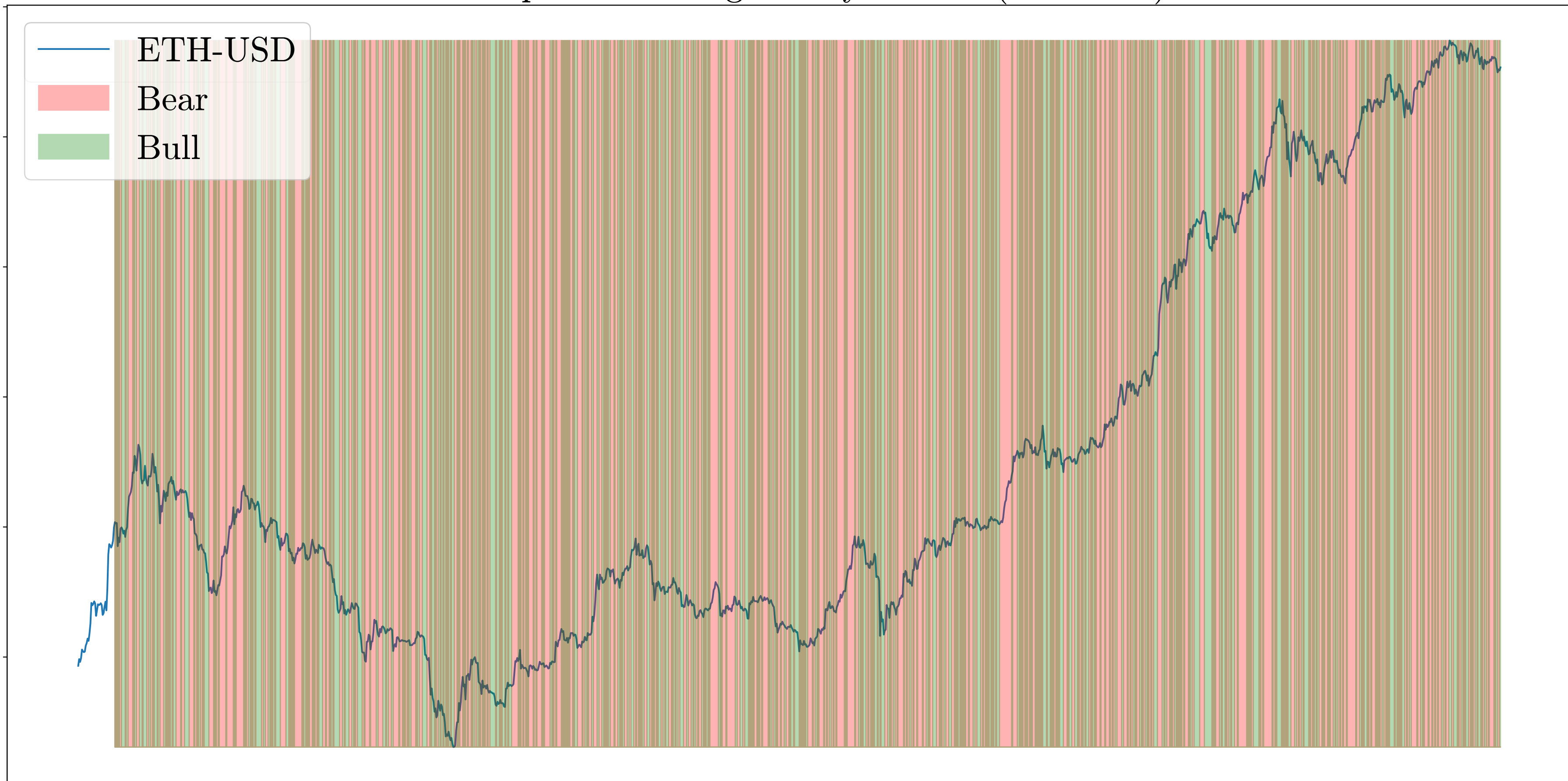
In-Sample Fitted Regimes by the JM ( \lambda=0.0001 )
