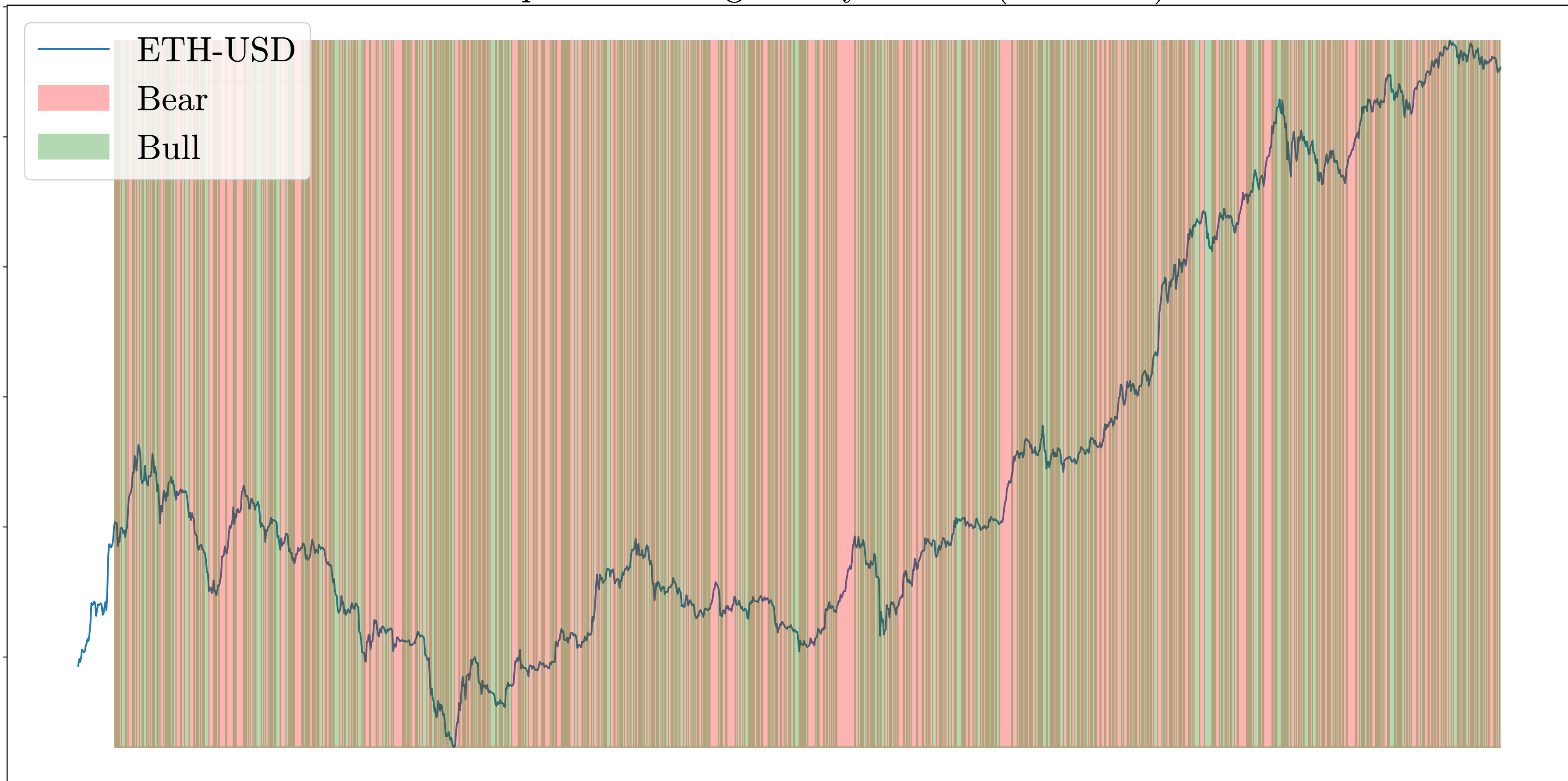
In-Sample Fitted Regimes by the JM ( \lambda=0.0003 )
