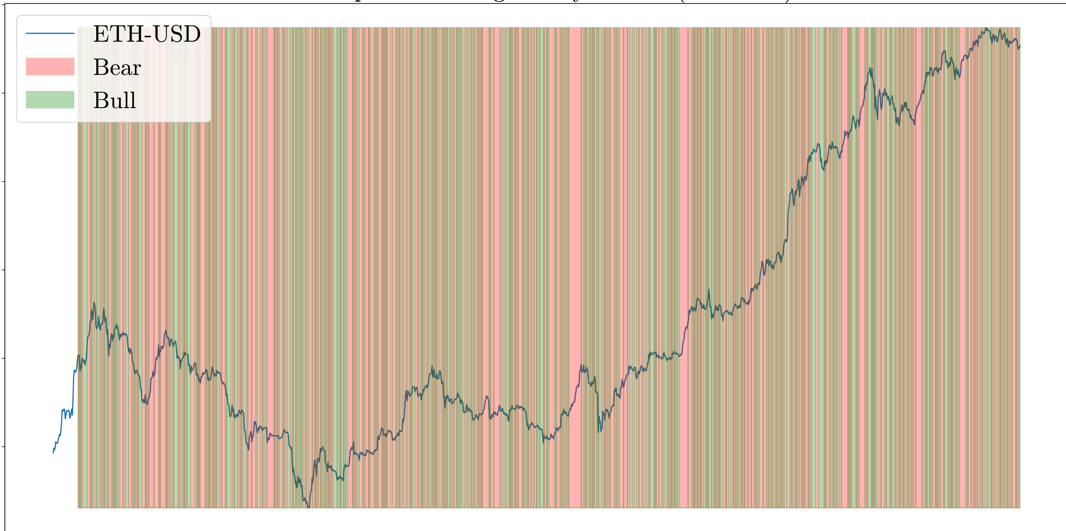
In-Sample Fitted Regimes by the JM ( \lambda=0.0004 )
