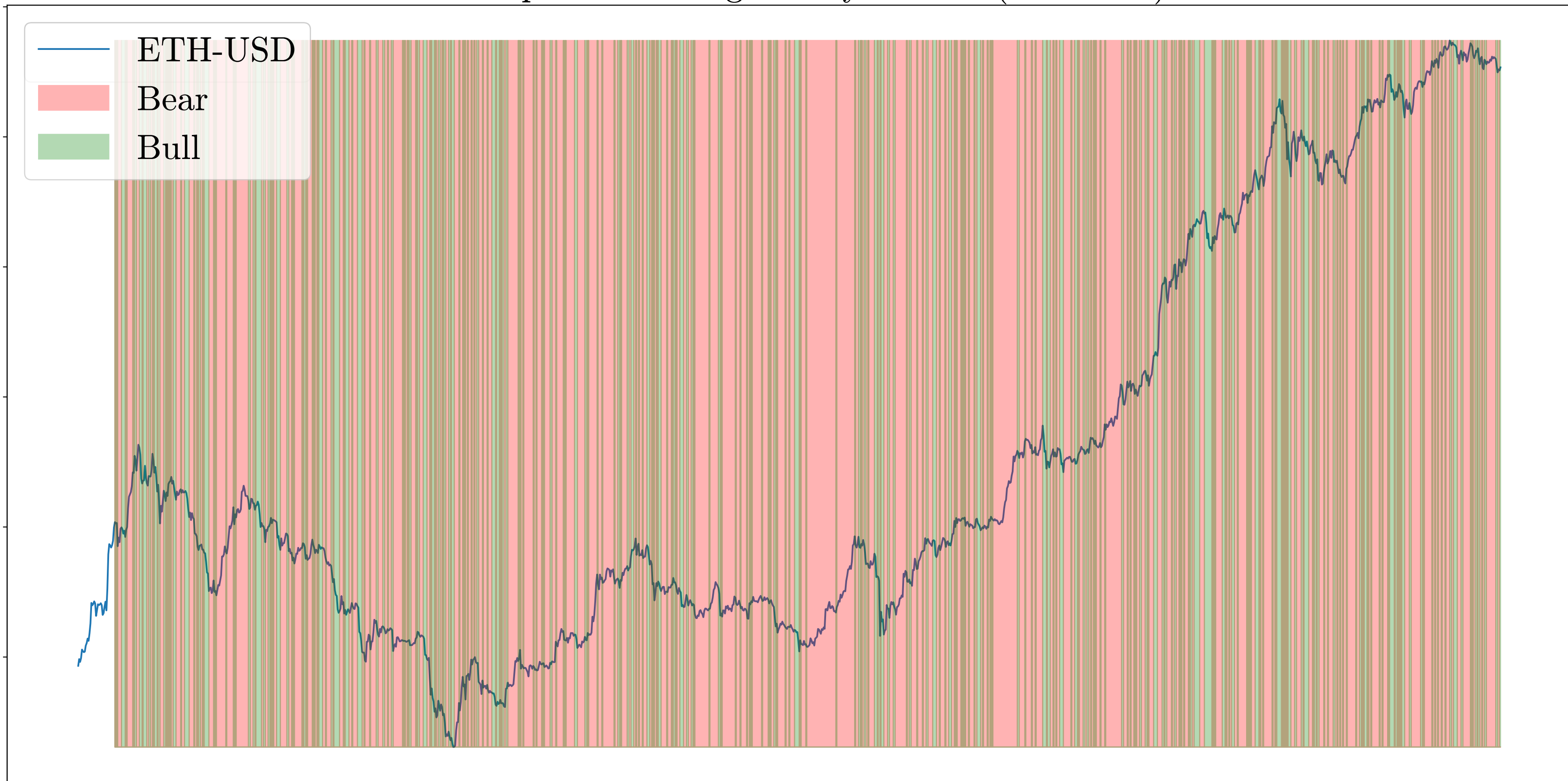
In-Sample Fitted Regimes by the JM ( \lambda=0.0008 )
