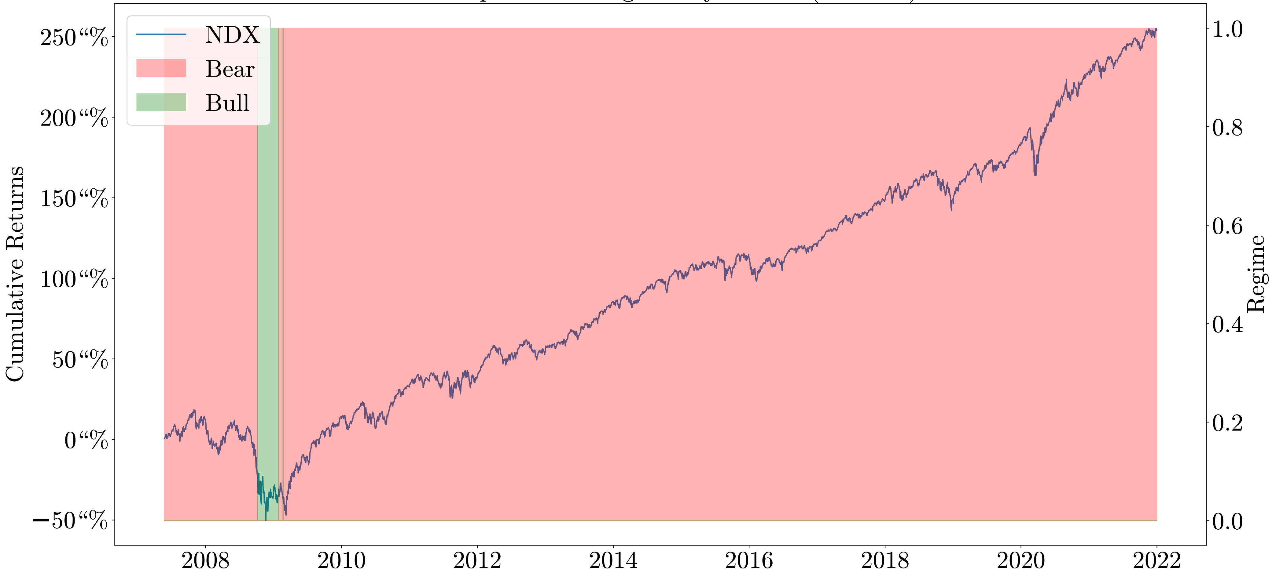
In-Sample Fitted Regimes by the JM ( \lambda=0.001 )
