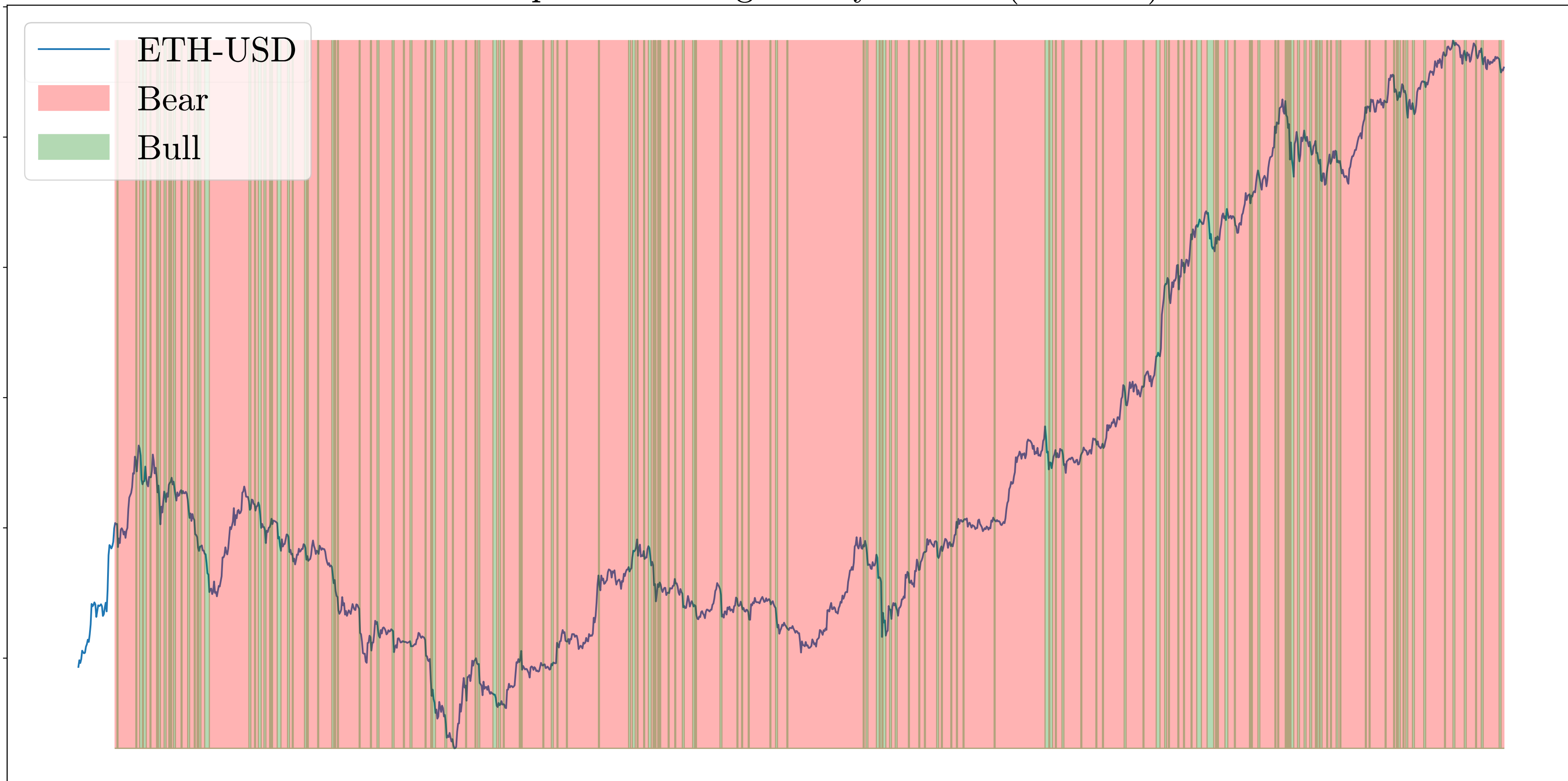
In-Sample Fitted Regimes by the JM ( \lambda=0.002 )
