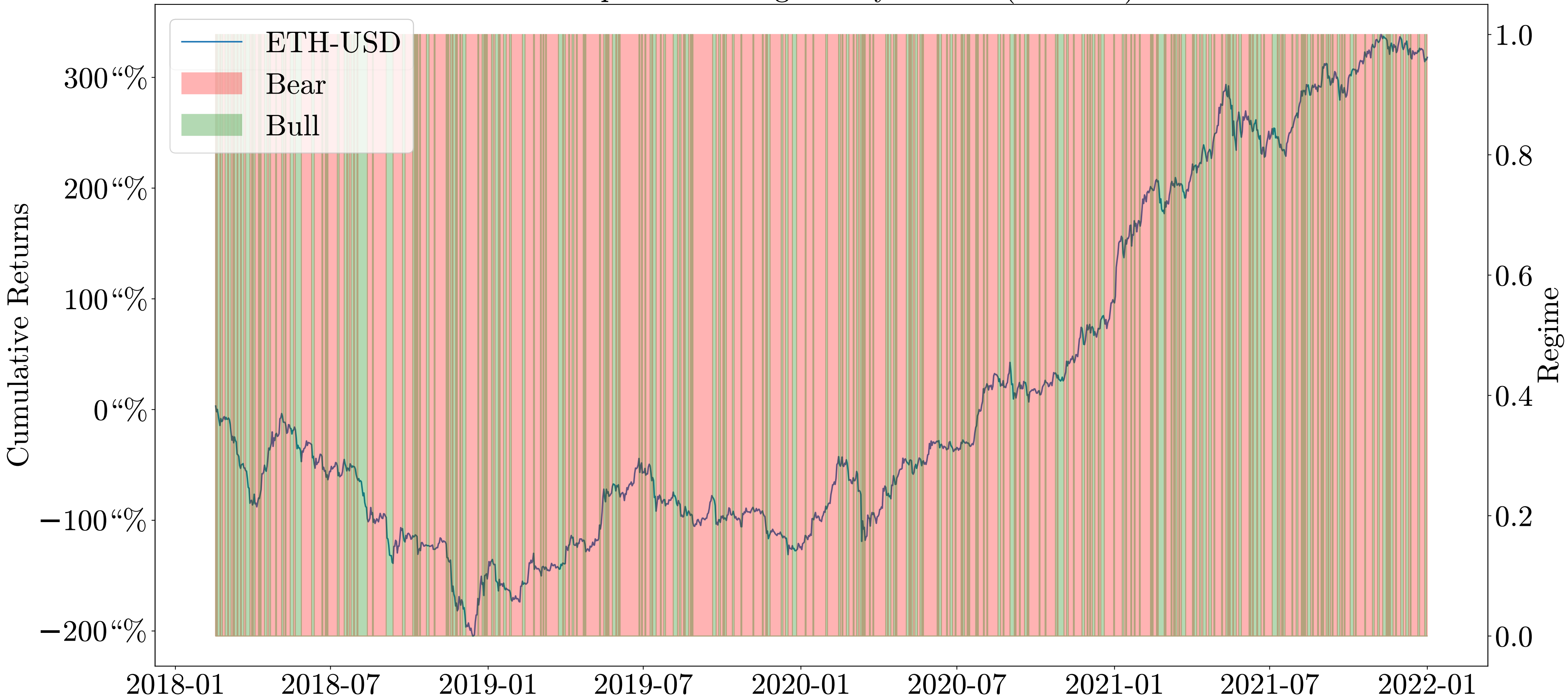
In-Sample Fitted Regimes by the JM ( \lambda=0.006 )
