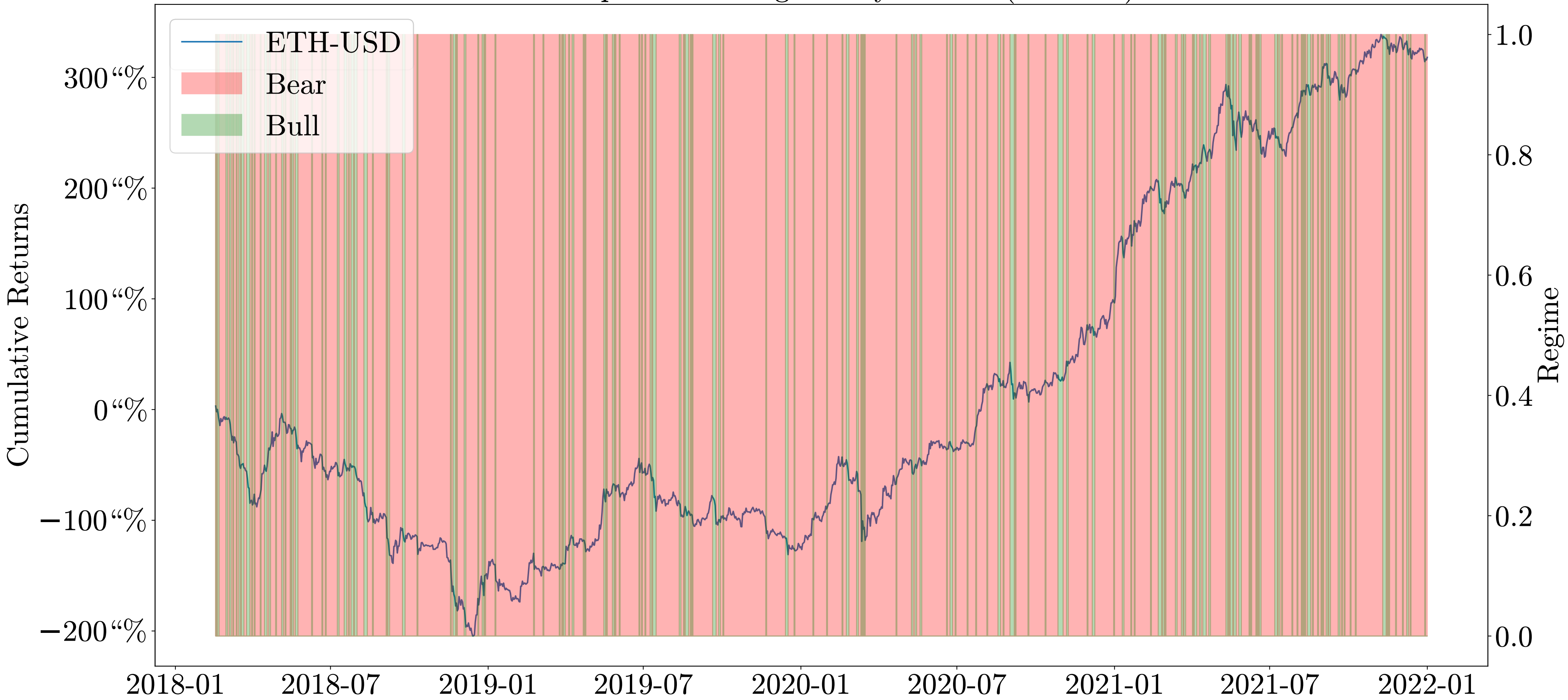
In-Sample Fitted Regimes by the JM ( \lambda=0.008 )
