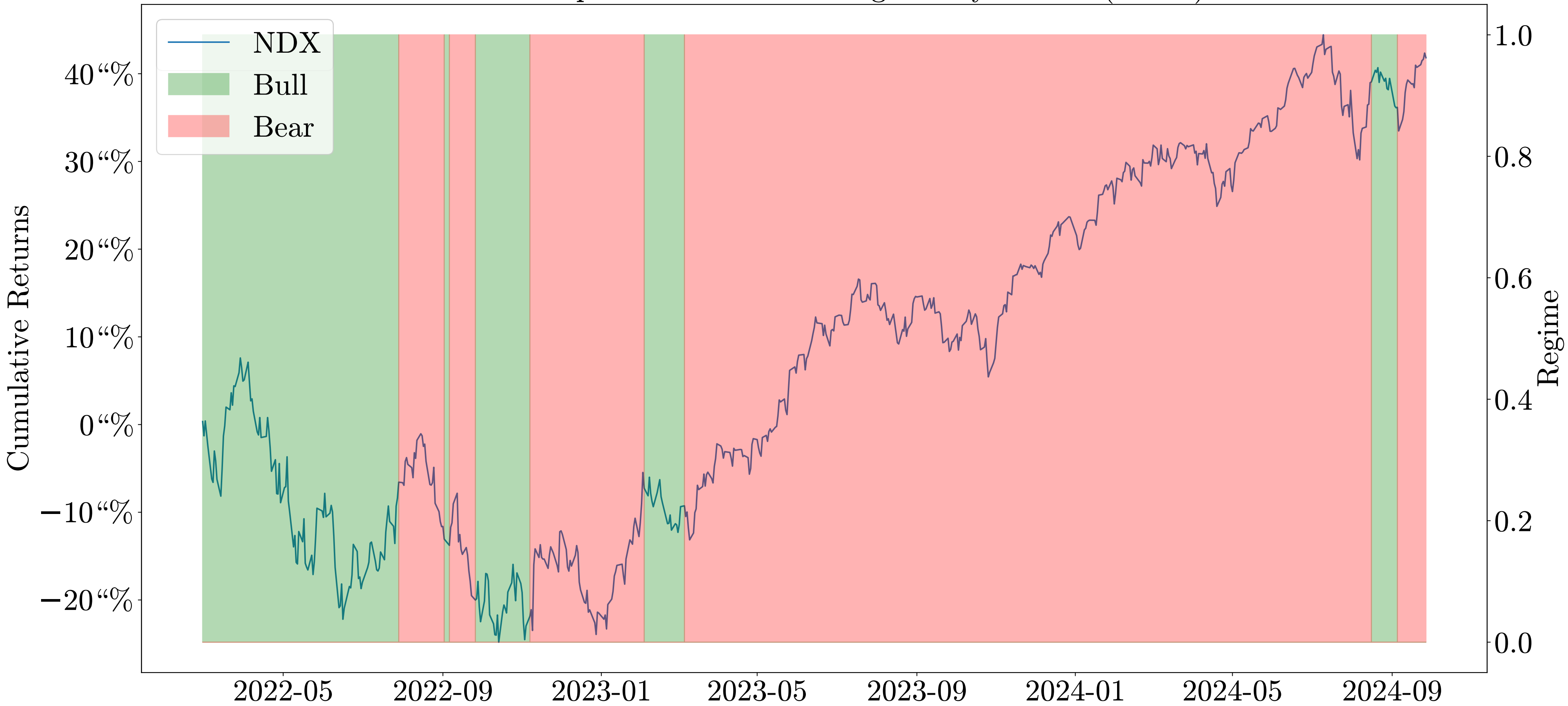
Out-of-Sample Online Inferred Regimes by the JM ( \lambda=0.0 )
